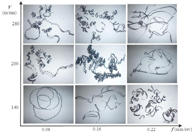
Fig. 5. Chip form for the different cutting combinaisons
