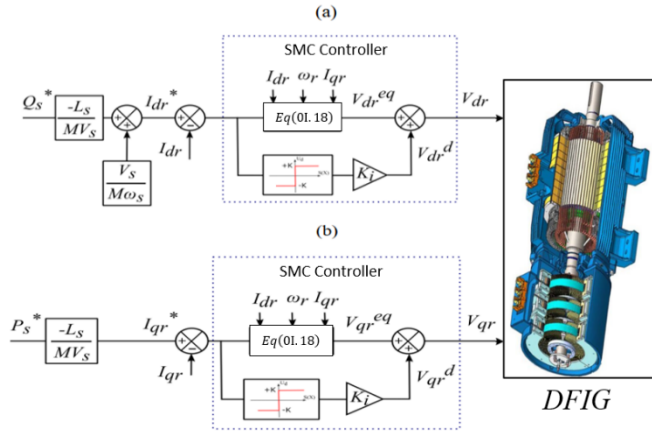
Figure 11. The DFIG control diagram with control (SMC): (a) Control of reactive power Q_s ; (b) Controls the active power P_s
