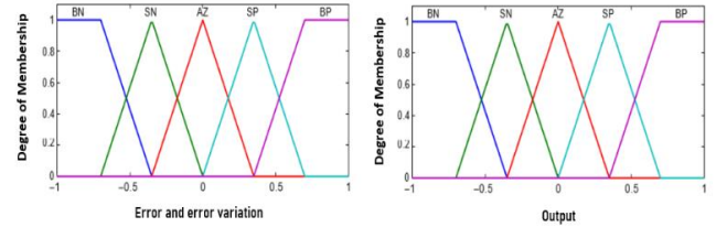
Figure 9. Description of fuzzy logic control in direct control of the DFIG
