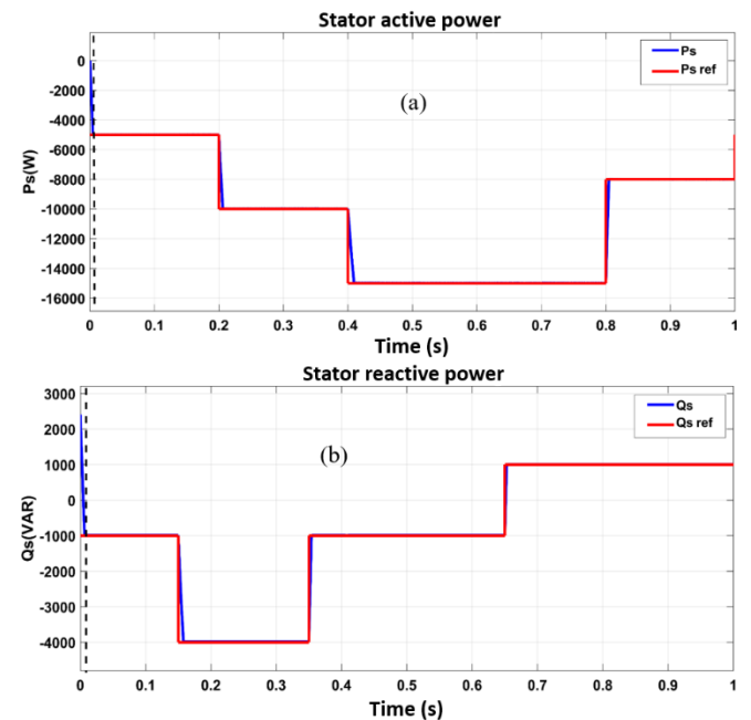
Figure 19. DFIG control simulation results with sliding mode controller: (a) Controls the active power P_s ; (b) Control of reactive power Q_s
