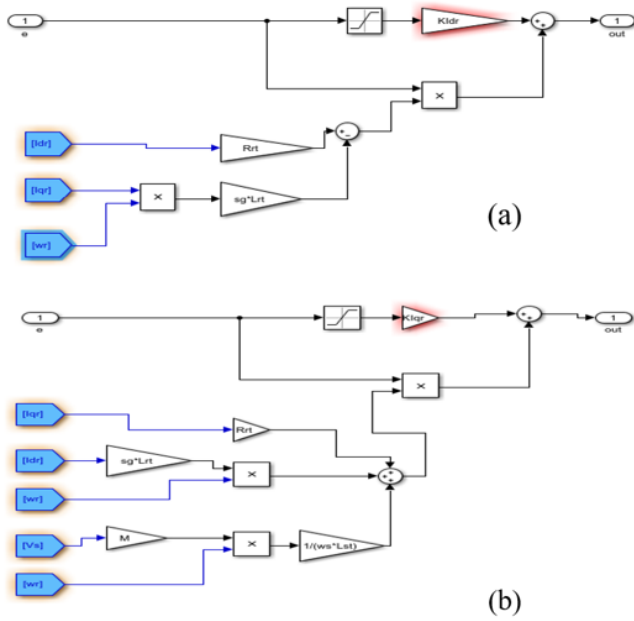
Figure 12. The DFIG control diagram with control (SMC): (a) Control of reactive power Q_s ; (b) Controls the active power P_s
