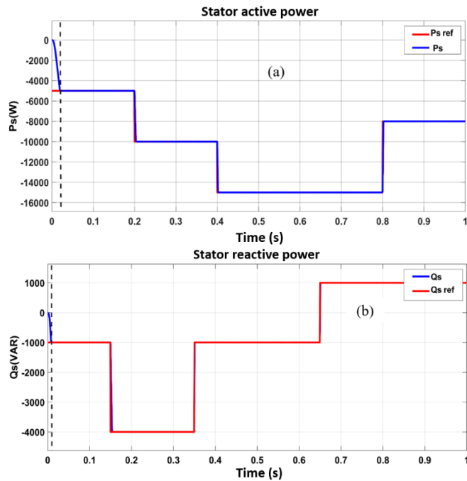
Figure 17. DFIG control simulation results with the fuzzy regulator using the direct method: (a) Controls the active power P_s ; (b) Control of reactive power Q_s
