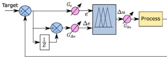
Figure 6. Synoptic diagram of a fuzzy regulator
