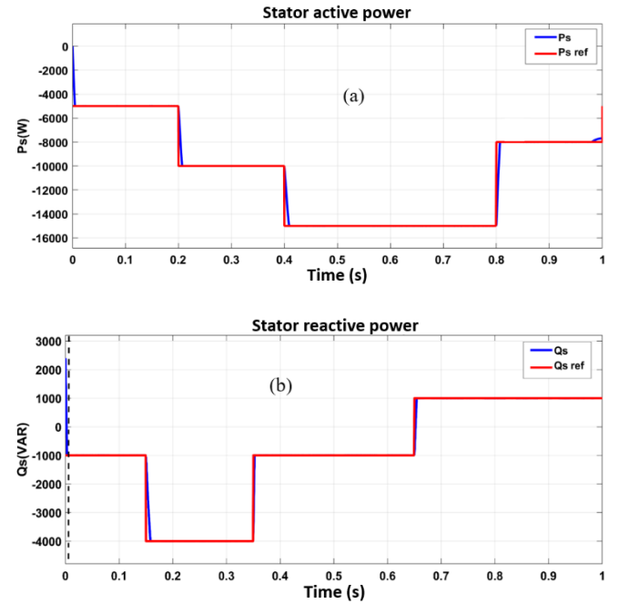
Figure 18. DFIG control simulation results with the fuzzy regulator using the indirect method: (a) Controls the active power P_s ; (b) Control of reactive power Q_s
