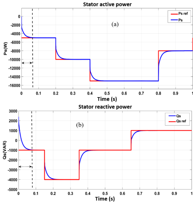
Figure 16. PI indirect method with power loop: (a) P_s ; (b) Q_s
