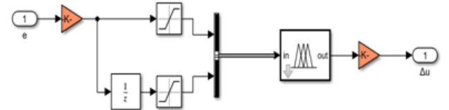
Figure 10. Description of the fuzzy logic control in the indirect control of the DFIG
