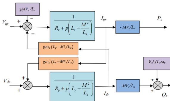
Figure 1. Used model of the DFIG
