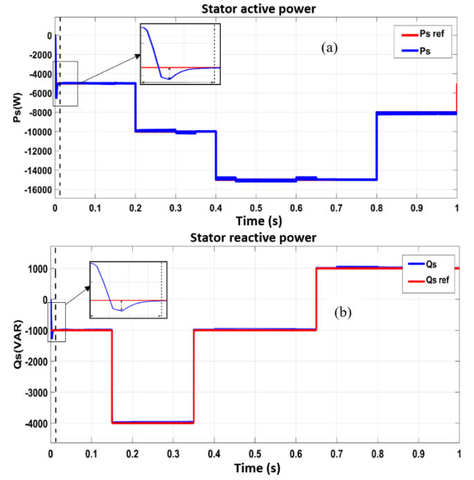
Figure 14. FIG control simulation results with the PI regulator using the direct method: (a) Controls the active power P_s ; (b) Control of reactive power Q_s
