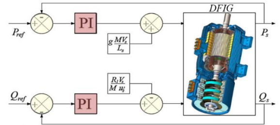
Figure 3. Block diagram of the direct control
