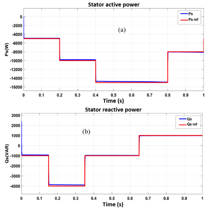
Figure 15. PI indirect method without power loop: (a) P_s ; (b) Q_s
