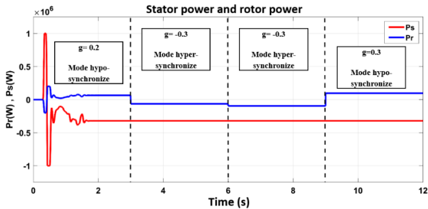
Figure 13. Simulation results of the DFIG model with different slip values
