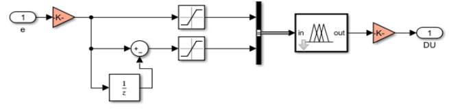
Figure 8. Block diagram of the fuzzy regulator used in direct control
