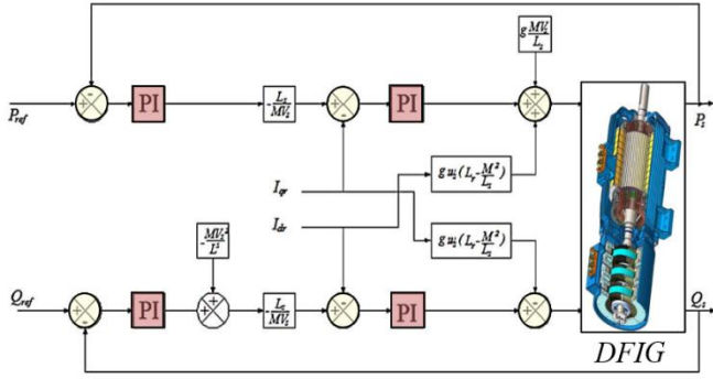
Figure 5. Block diagram of indirect control with power loop
