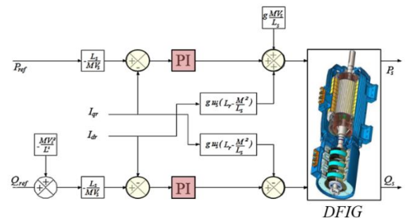
Figure 4. Block diagram of indirect control without power loop
