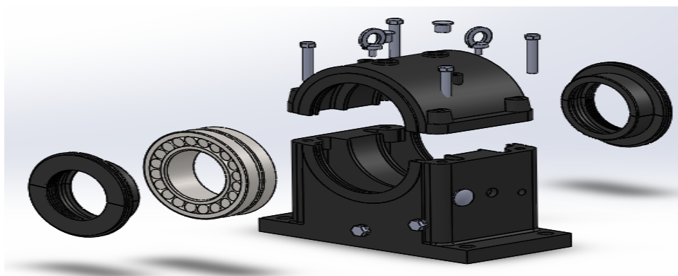
Fig. 3 Exploded view of the fixed bearing
